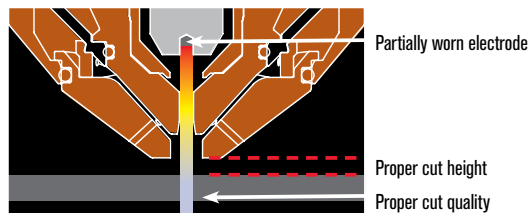
Consumable life and cut quality optimized
