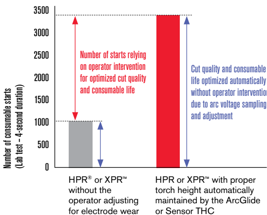
Number of consumable starts with < 0.25 mm (0.010") deviation from proper cut height without operator intervention (130 A) 12 mm (1/2") mild steel
